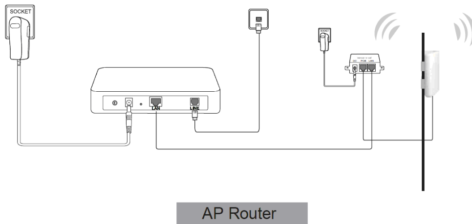
Figure 2-2 Hardware Installation of the WAB-6121 in AP Router mode
