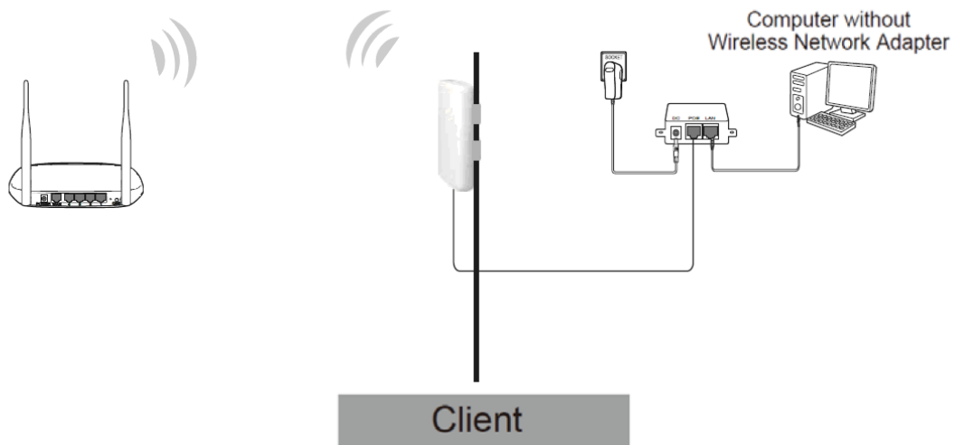
Figure 2-7 Hardware Installation of the WAB-6121 in Client mode
