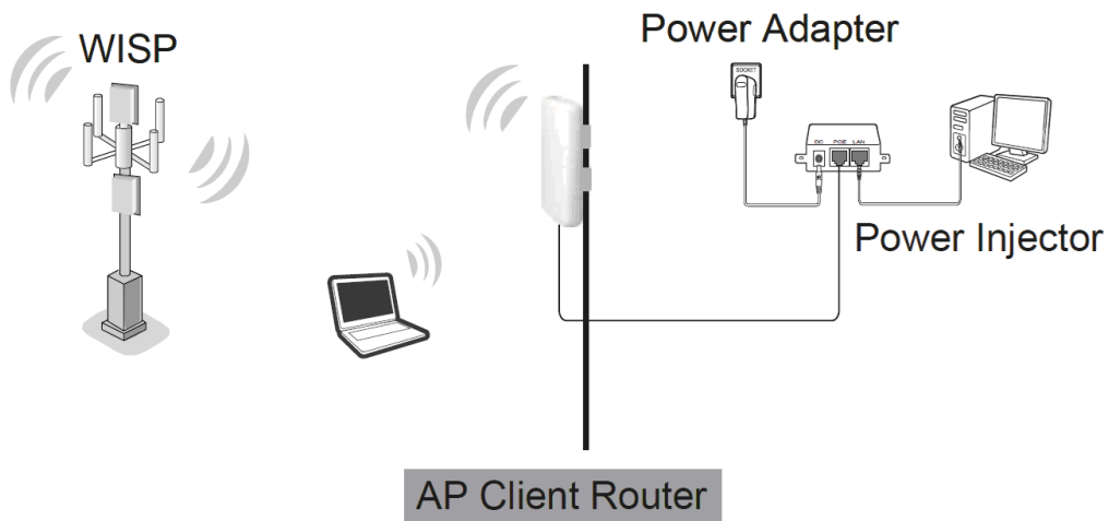
Figure 2-1 Hardware Installation of the WAB-6121 in AP Client Router mode
