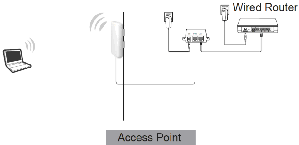
Figure 2-3 Hardware Installation of the WAB-6121 in Access Point mode
