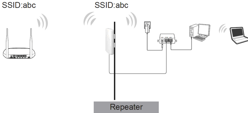
Figure 2-5 Hardware Installation of the WAB-6121 in (Universal) Repeater mode
