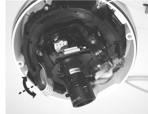
Tilt Adjustment
