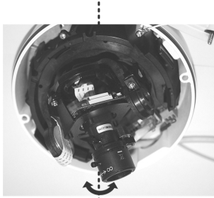
Pan Adjustment
