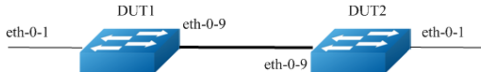
Figure 12-13 Tpoam Topology
