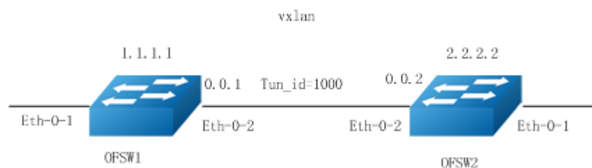
Figure 12-23 Vxlan Tunnel topology
