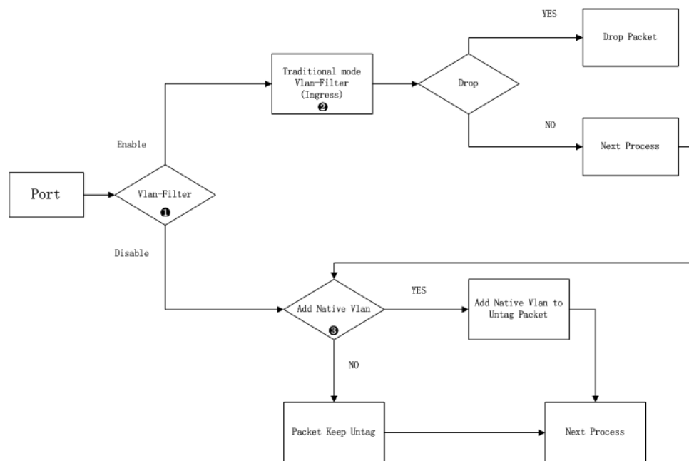
Figure 12-2 Hybrid inport forwarding structure topology
