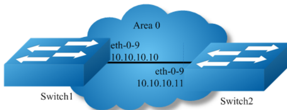
Figure 5-2 ospf
