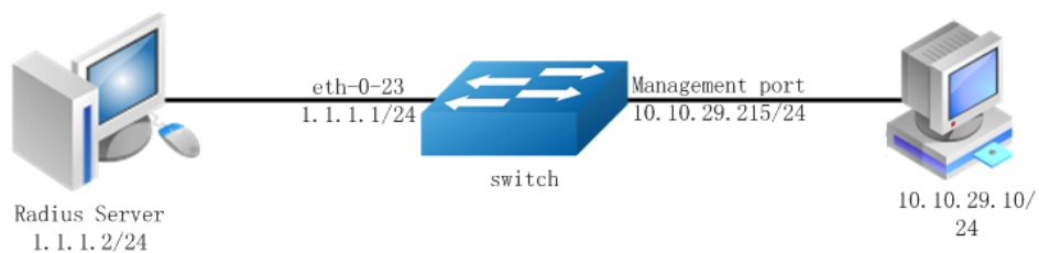
Figure 6-1 RADIUS authentication application
