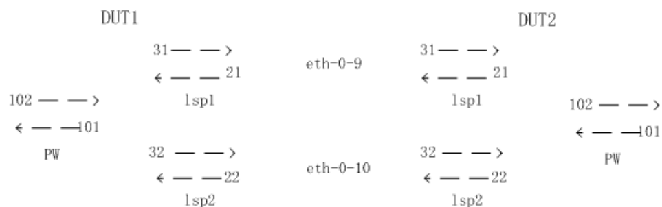
Figure 12-18 LSP APS topology
