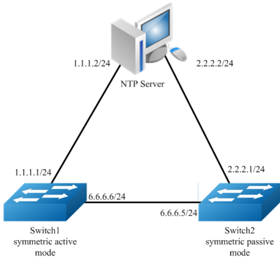
Figure 8-2 NTP symmetric mode
