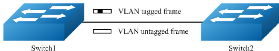
Figure 3-7 Trunk link
