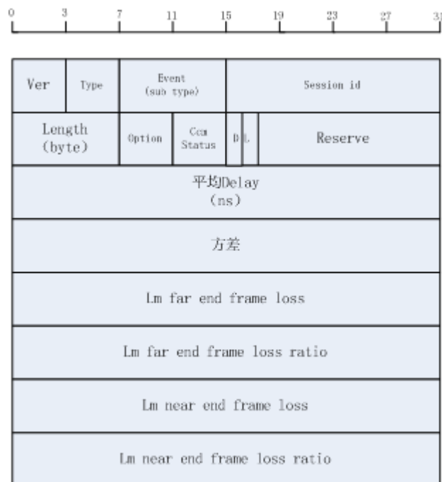
Figure 12-15 Oam Cycle Message Structure
