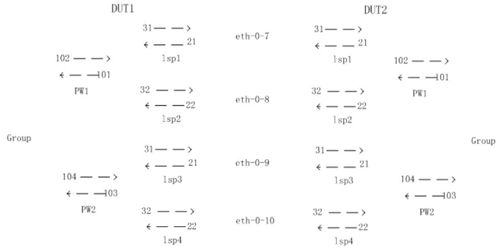
Figure 12-20 PW APS With LSP APS topology
