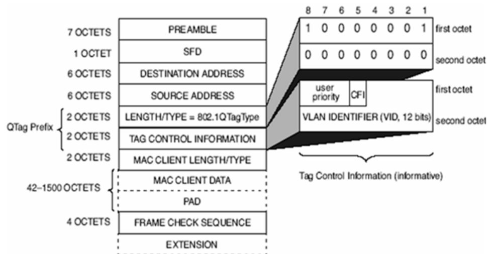
Figure 3-6 Tagged Frame
