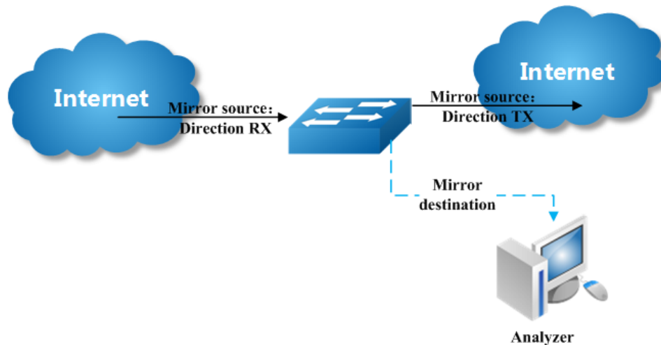
Figure 7-3 Mirror
