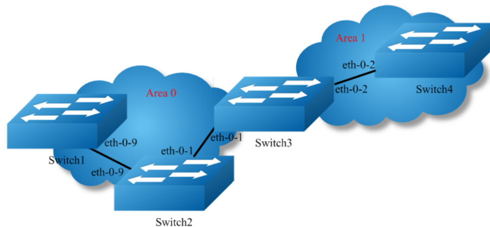
Figure 5-4 ospf authentication
