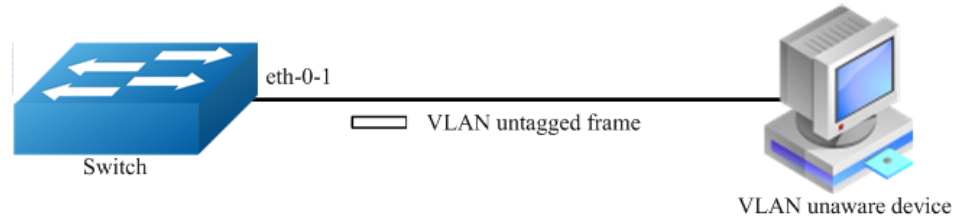
Figure 3-9 Access link
