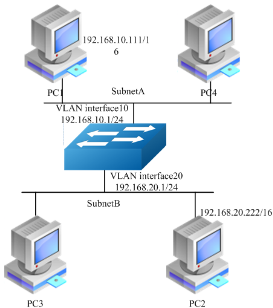
Figure 4-4 arp proxy
