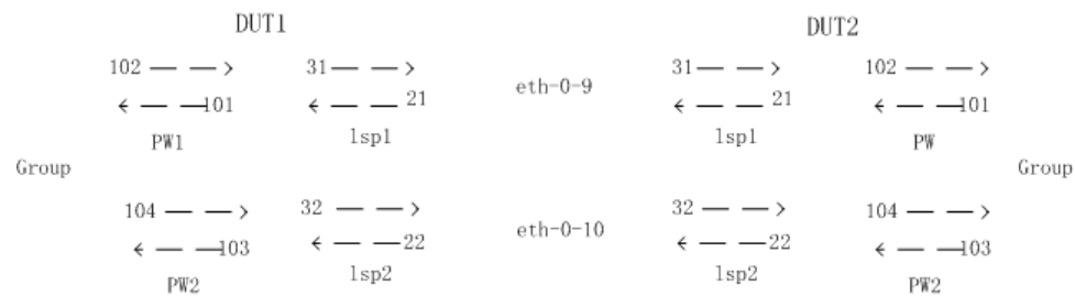
Figure 12-19 PW APS Without LSP APS topology
