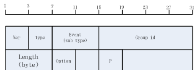
Figure 12-21 ASP-Group Message Structure
