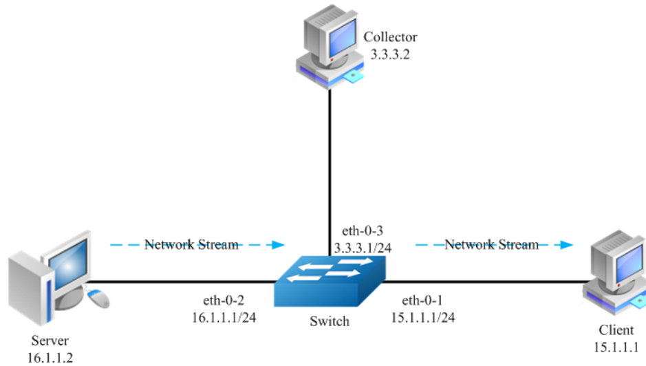
Figure 8-6 sflow
