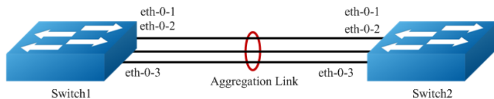
Figure 3-12 Static Agg
