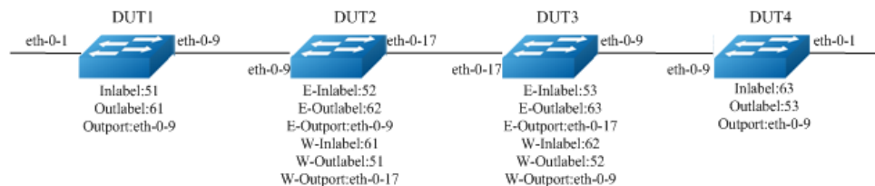
Figure 12-14 Tpoam loopback Topology
