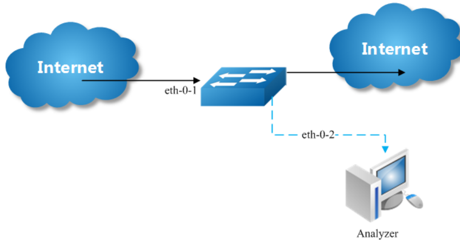
Figure 7-4 port Mirror
