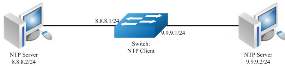
Figure 8-4 NTP
