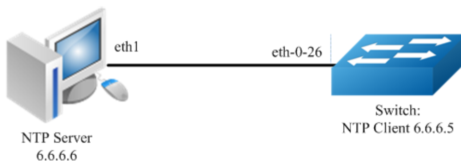
Figure 8-1 NTP
