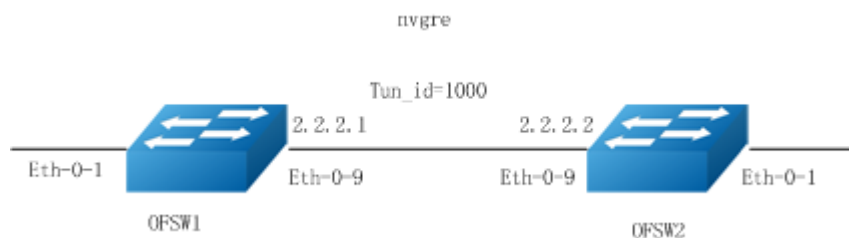
Figure 12-28 nvgre Tunnel topology
