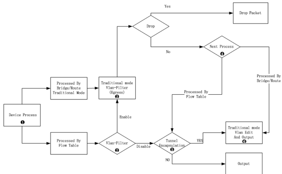
Figure 12-3 Hybrid Output forwarding structure topology
