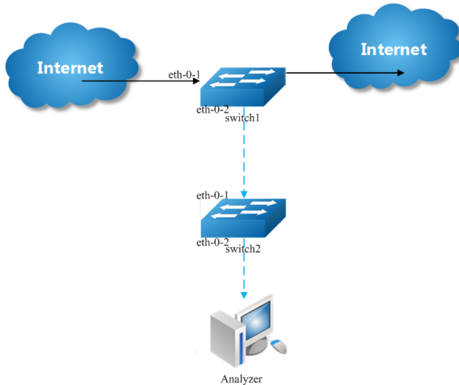
Figure 7-6 Remote Mirror
