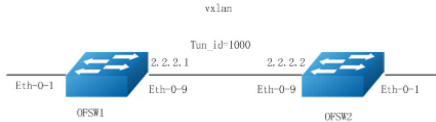
Figure 12-24 Vxlan Tunnel topology
