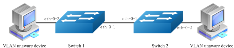
Figure 3-10 Trunk link
