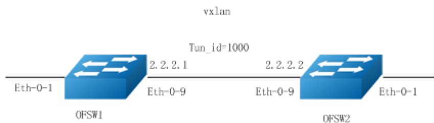
Figure 12-26 l2gre Tunnel topology
