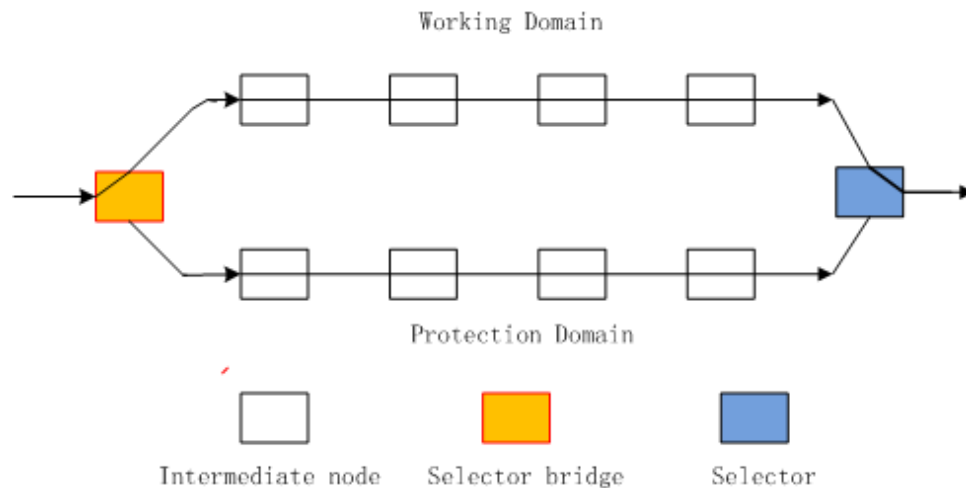
Figure 12-17 G8131 basic topology
