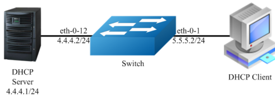
Figure 4-7 DHCP relay
