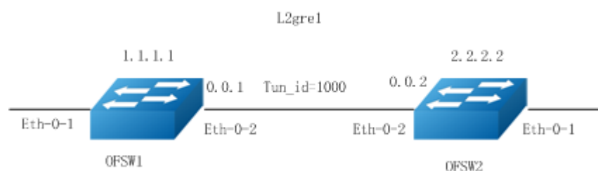
Figure 12-25 l2gre Tunnel topology
