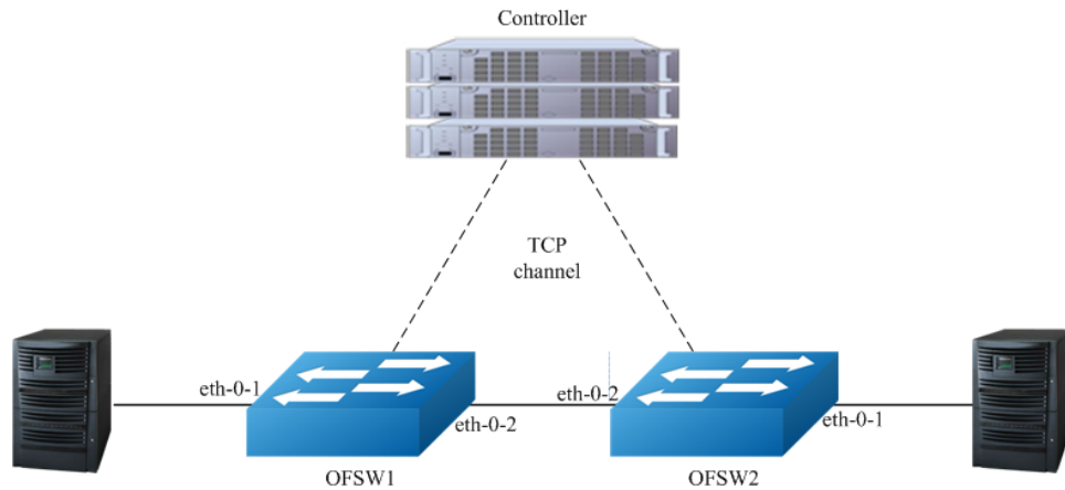
Figure 12-7 Hybrid Openflow Table topology
