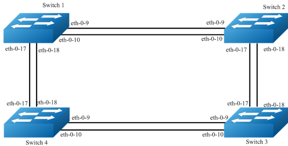
Figure 3-13 RSTP
