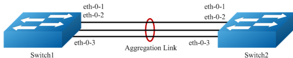
Figure 3-11 LACP
