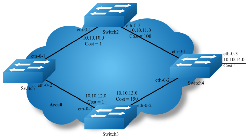
Figure 5-3 ospf cost
