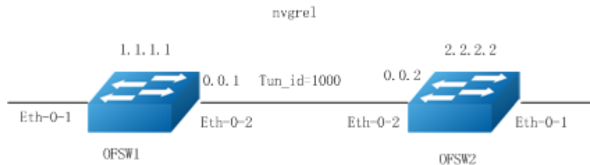
Figure 12-27 nvgre Tunnel topology
