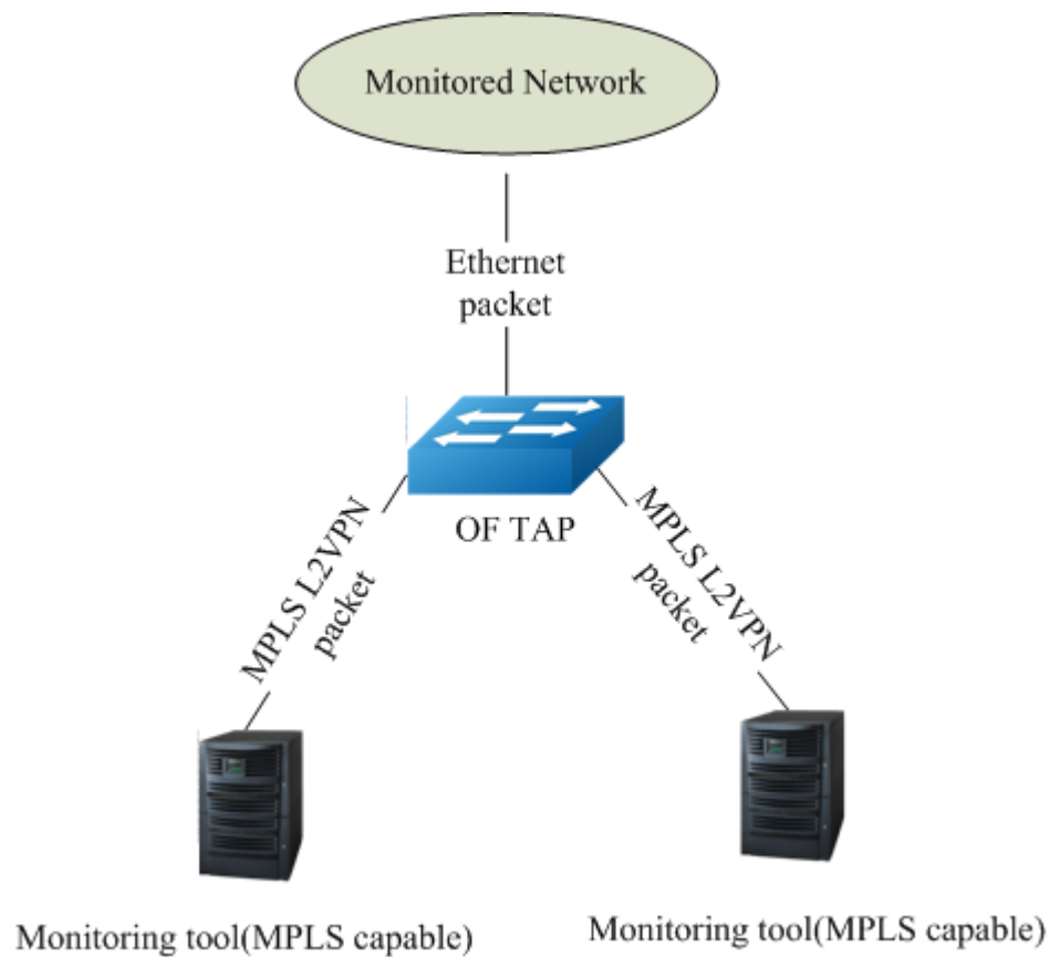
Figure 12-22 Add Flex-Mpls Header Topology
