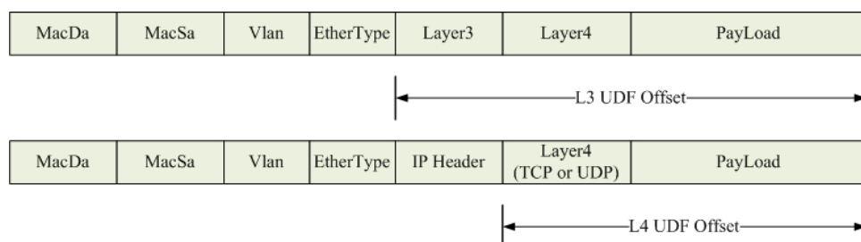
Figure 12-32 L3/L4 offset type in packet
