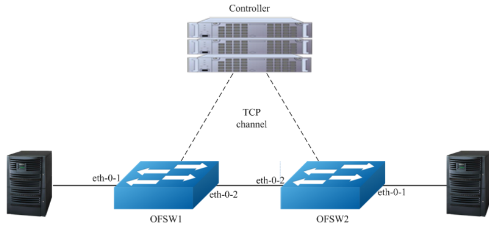
Figure 12-6 Hybrid Openflow Table topology
