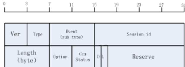
Figure 12-16 Oam Interrupt Message Structure
