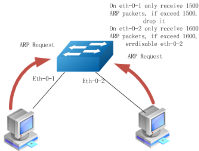
Figure 4-3 ARP Rate limit
