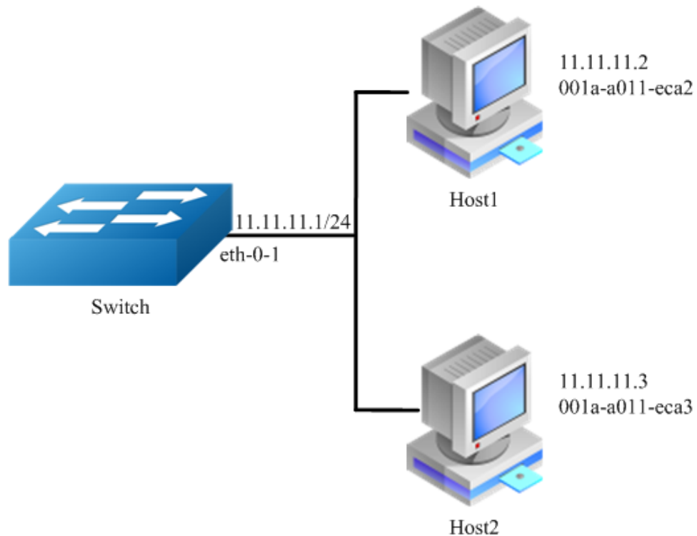
Figure 4-1 arp
