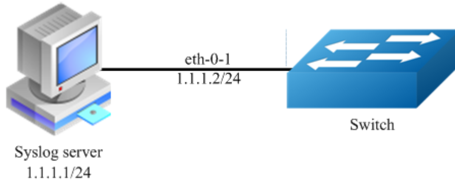
Figure 7-1 syslog server
